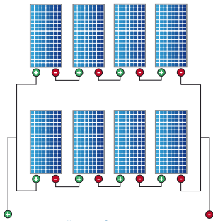
Installation for 48V pump (Four 17.5V panels connected in series)
